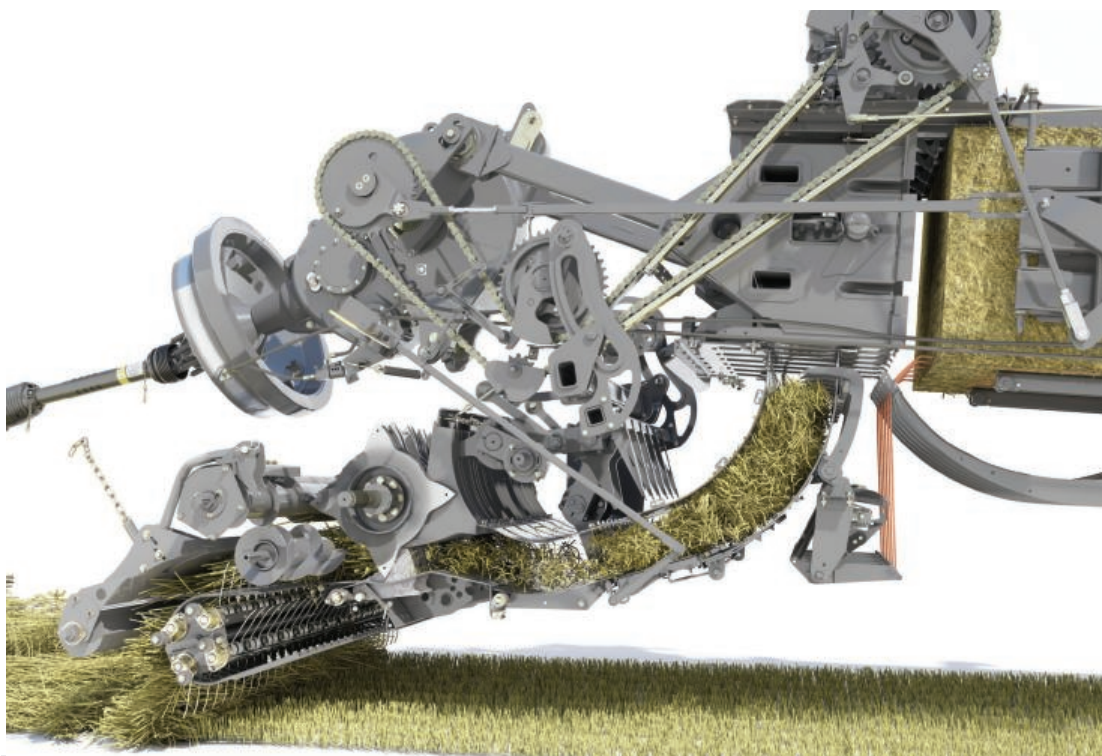
Pre-Compression Chamber - filling.
