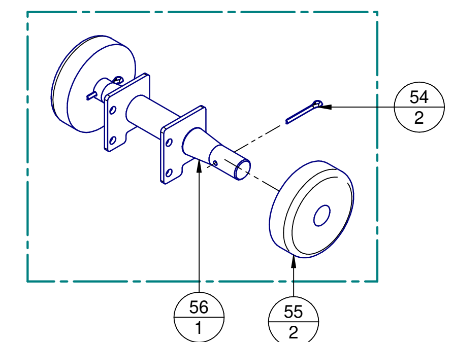
Tapered Shaft Designed Extension Shaft CHK Transtackers
